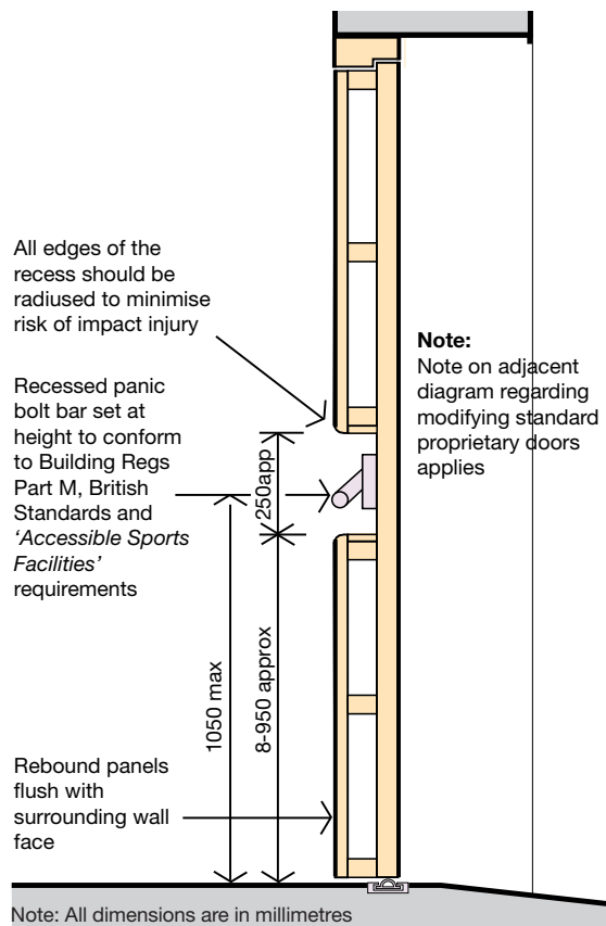
External escape doors must be panelled out to line through with the wall surface. The lower section can then form part of the five-a-side football rebound zone (1.21m high along walls) and a flush facing is essential for overall safety.
